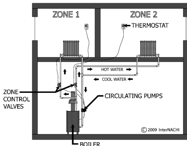
ZONE CONTROL WITH VALVES
