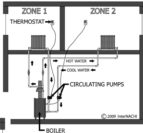
ZONE CONTROL WITH PUMPS
